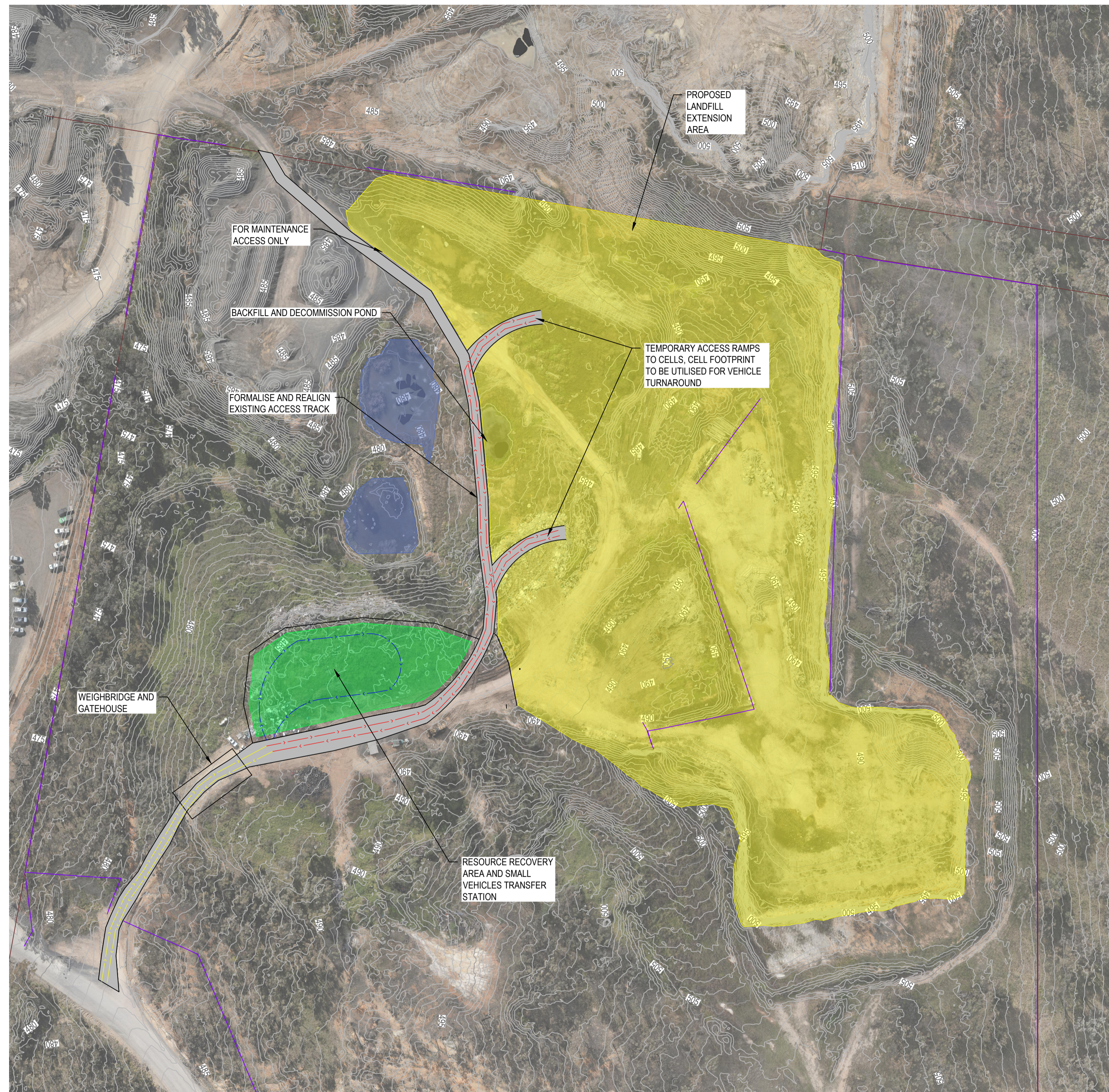
SITE LAYOUT PLAN SCALE 1:1000
